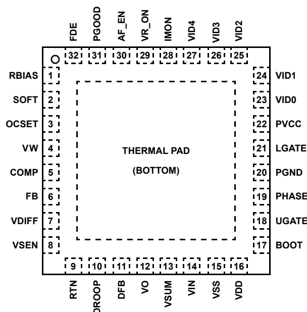
ISL6263B (32 LD 5x5 QFN) TOP VIEW
