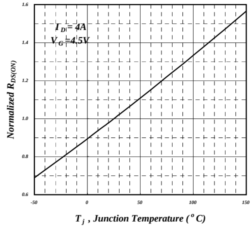
Fig 4. Normalized On-Resistance
