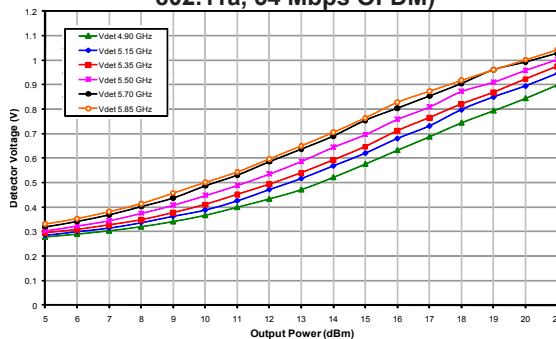
Figure 24: Voltage Detector vs. Output Power Across Frequency ( V_{cc} = +3.3\text{ V} , Temp = +25\text{ }^{\circ}\text{C} , 802.11a, 54 Mbps OFDM)
