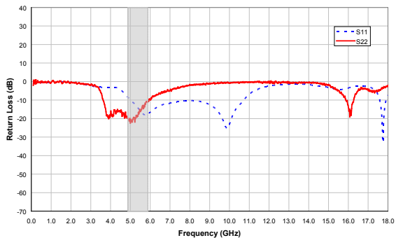
Figure 32: Tx Path S11 and S22 Return Loss (Vcc = +3.3 V, Temp = +25 °C)
