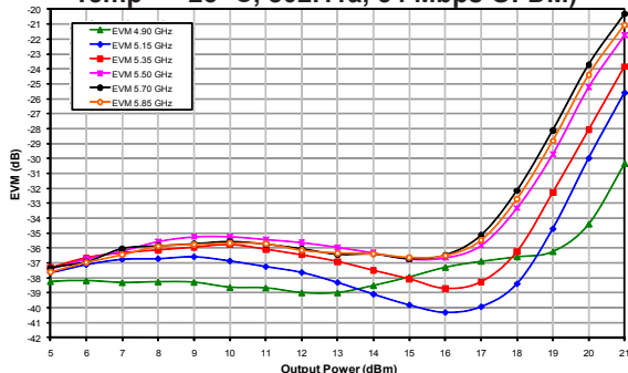
Figure 20: Tx Path Dynamic EVM vs. Output Power Across Frequency (Vcc = +3.0 V, Temp = +25 °C, 802.11a, 54 Mbps OFDM)
