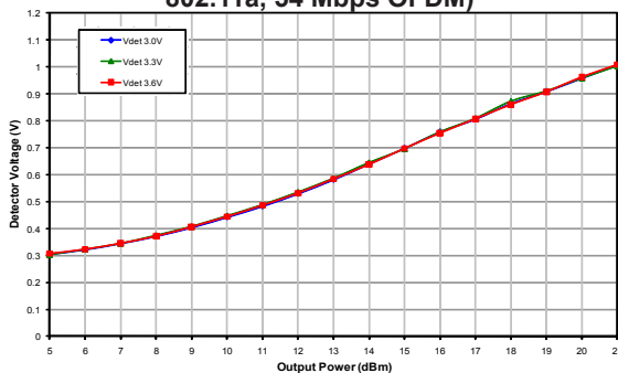
Figure 25: Voltage Detector vs. Output Power Across Voltage (Freq = 5.5 GHz, Temp = +25\text{ }^{\circ}\text{C} , 802.11a, 54 Mbps OFDM)
