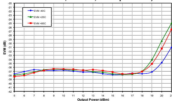
Figure 19: Tx Path Dynamic EVM vs. Output Power Across Temperature (Freq = 5.5 GHz, Vcc = +3.3 V, 802.11a, 54 Mbps OFDM)
