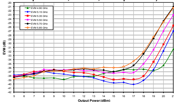
Figure 23: Tx Path Dynamic EVM vs. Output Power Across Frequency ( V_{cc} = +3.3\text{ V} , Temp = +85\text{ }^{\circ}\text{C} , 802.11a, 54 Mbps OFDM)
