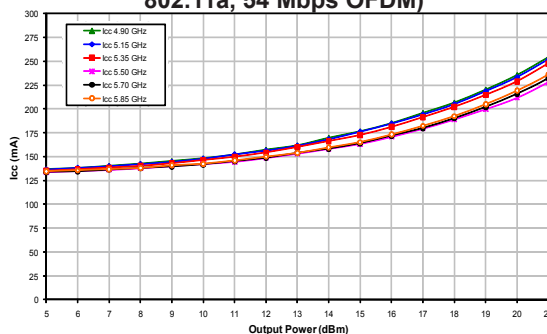
Figure 10: Tx Path Icc vs. Output Power Across Frequency (Vcc = +3.3V, Temp = +25 °C 802.11a, 54 Mbps OFDM)
