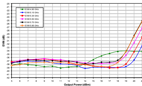
Figure 22: Tx Path Dynamic EVM vs. Output Power Across Frequency ( V_{cc} = +3.3\text{ V} , Temp = -40\text{ }^{\circ}\text{C} , 802.11a, 54 Mbps OFDM)
