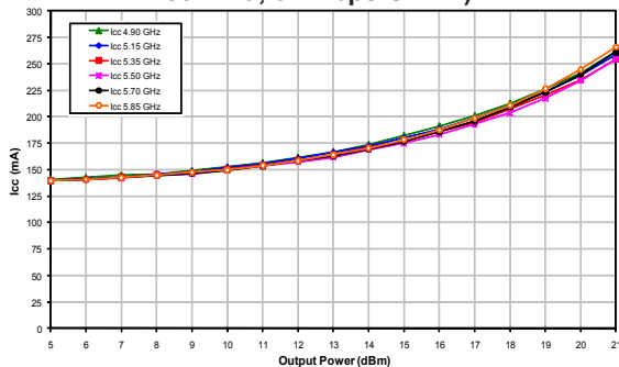
Figure 16: Tx Path Icc vs. Output Power Across Frequency (Vcc = +3.3 V, Temp = +85 °C 802.11a, 54 Mbps OFDM)
