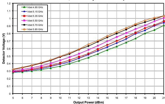
Figure 28: Voltage Detector vs. Output Power Across Frequency (Vcc = +3.6 V, Temp = +25 °C 802.11a, 54 Mbps OFDM)
