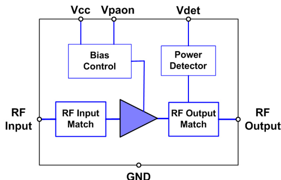
Figure 1: Block Diagram and Pinout
