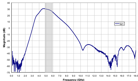
Figure 31: Tx Path S21 Response (Vcc = +3.3V, Temp = +25 °C)
