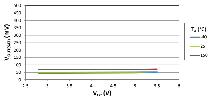
Average Low Output Voltage versus Supply Voltage for I_{OUT} = 5 mA
