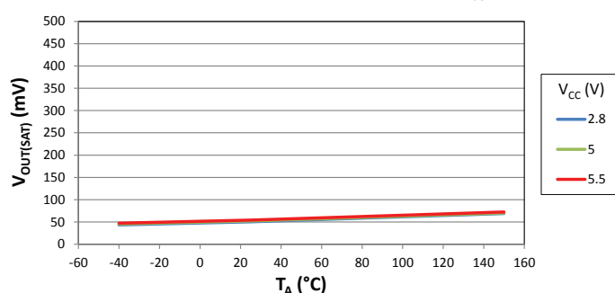
Average Low Output Voltage versus Ambient Temperature for I_{OUT} = 5 mA
