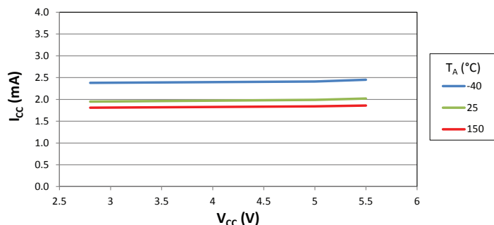
Average Supply Current versus Supply Voltage
