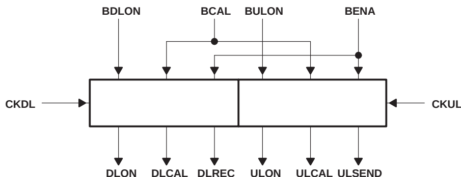
Figure 17. Timing Interface
