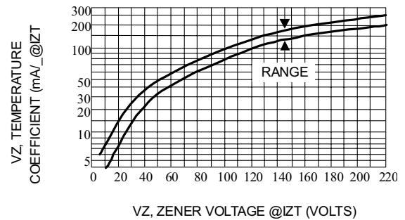
Fig. 2-TEMPERATURE COEFFICIENT-RANGE FOR UNITS 6 TO 51 VOLTS
