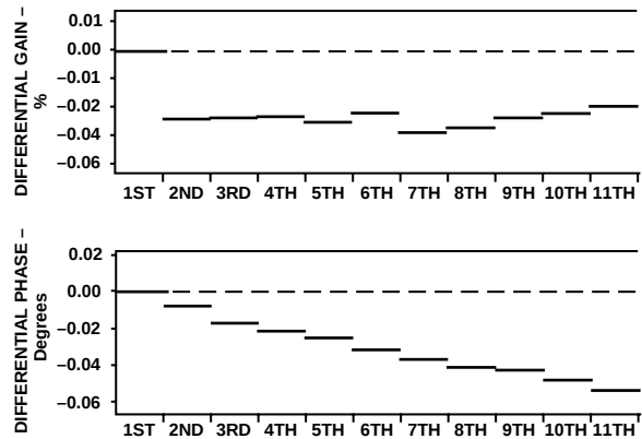
Figure 18. Differential Gain and Phase Error, G = 2 , NTSC Input Signal, R_L = 1k\Omega , V_S = 5V
