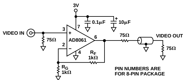
Figure 49. Single 3 V Sync Stripper Using AD8061
