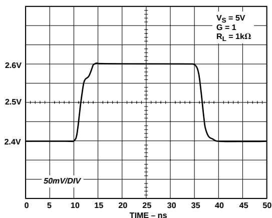
Figure 39. 200 mV Step Response
