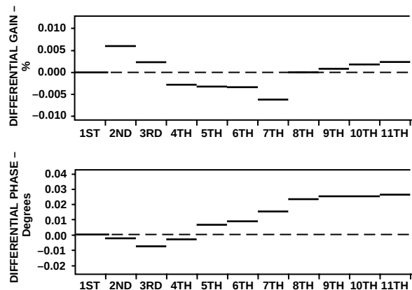
Figure 19. Differential Gain and Phase Error, G = 2 , NTSC Input Signal, R_L = 150\Omega , V_S = 5V
