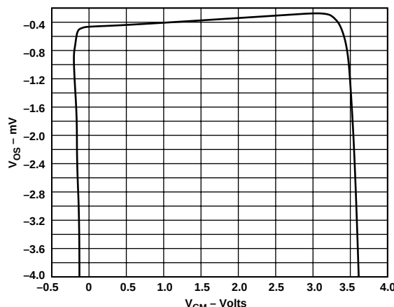
Figure 41. V_{OS} vs. Common-Mode Voltage, V_S = 5 V
