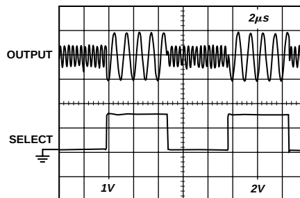
Figure 53. AD8063 Mux Output
