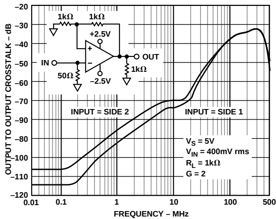
Figure 28. AD8062 Crosstalk, V_{OUT} = 2.0 V p-p, R_L = 1 k \Omega , G = 1 , V_S = 5 V
