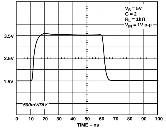
Figure 36. 1 V Step Response
