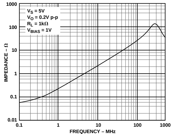
Figure 32. Output Impedance vs. Frequency, V_{OUT} = 0.2 V p-p, R_L = 1 k \Omega , V_S = 5 V
