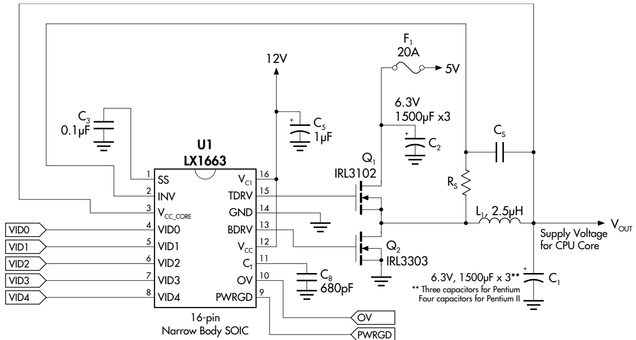
FIGURE 8 — Pentium II Processor Application With OVP, Power Good And Loss-Less Current Sensing (Synchronous)
