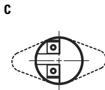
VERTICAL - Both terminals extend up and away, on a perpendicular plane to the mounting bracket / base
