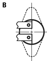
PARALLEL - Terminals on same side of thermostat, on a parallel plane to the mounting bracket / base
