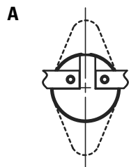
OPPOSED - Terminals on opposite sides of thermostat, on a parallel plane to the mounting bracket / base
