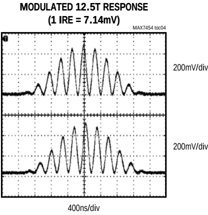
Typical Operating Characteristics (continued) (R LOAD = 150Ω to GND, V CC = +5V, and T A = +25°C.)
