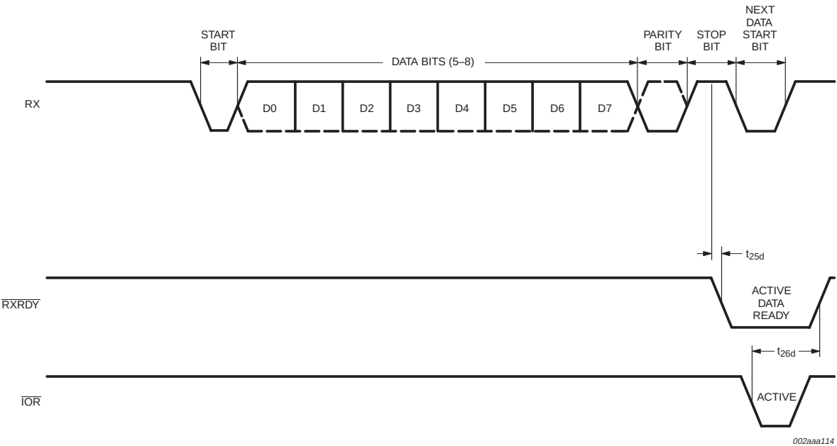
Fig 16. Receive ready timing in non-FIFO mode.
