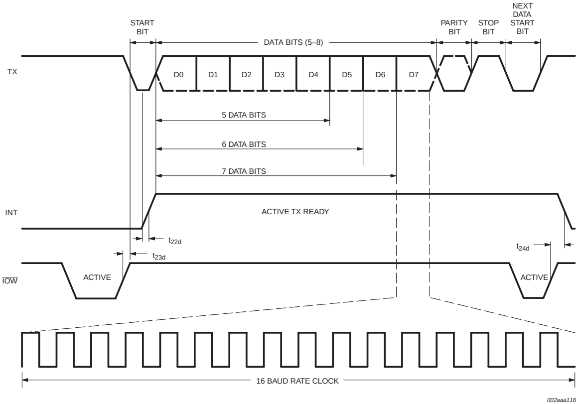
Fig 18. Transmit timing.
