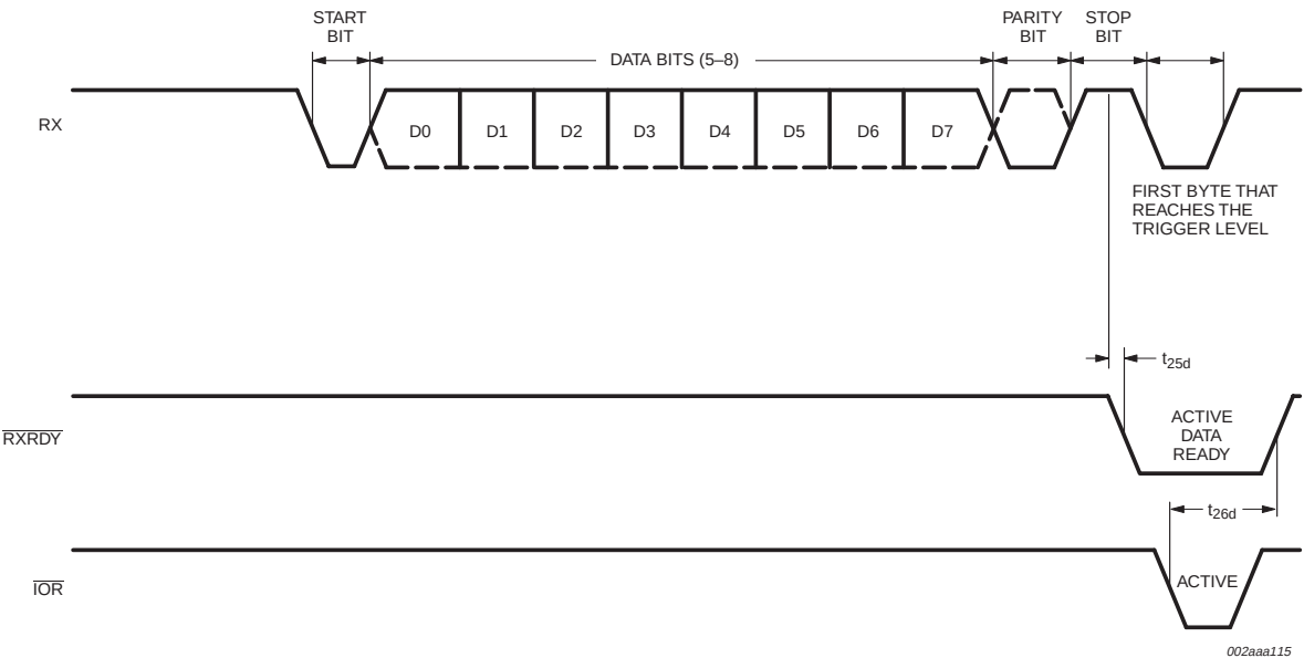
Fig 17. Receive ready timing in FIFO mode.
