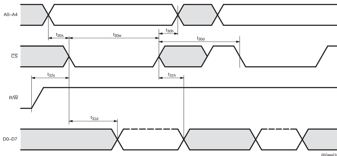
Fig 9. General read timing in 68 mode.
