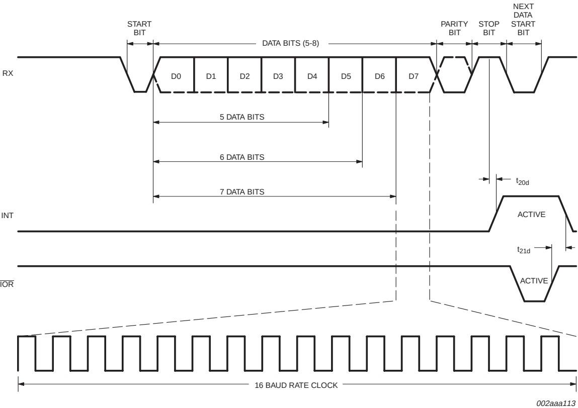
Fig 15. Receive timing.
