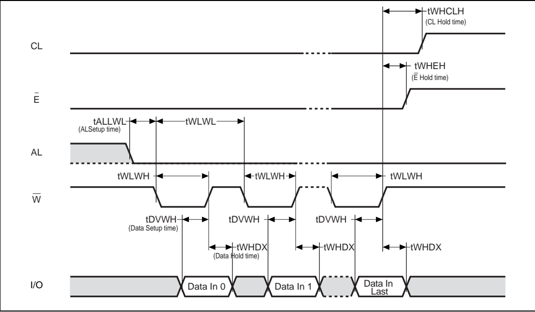
Figure 23. Data input latch AC waveforms
