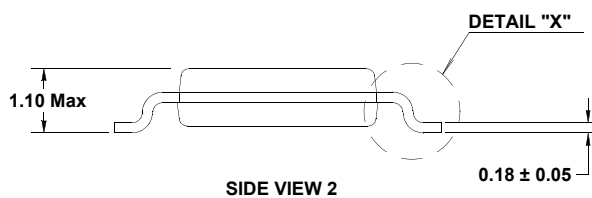
SIDE VIEW 2
