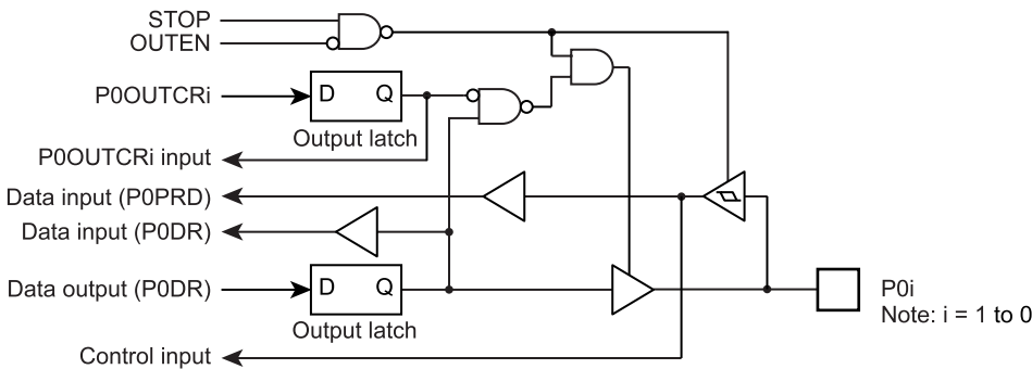
Figure 5-2 Port P0
