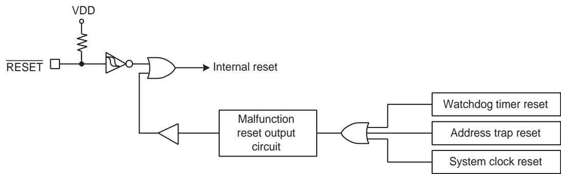
Figure 2-14 Reset Circuit
