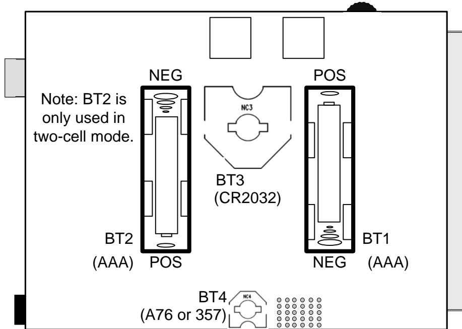
Figure 8. Bottom of C8051F912 Target Board
