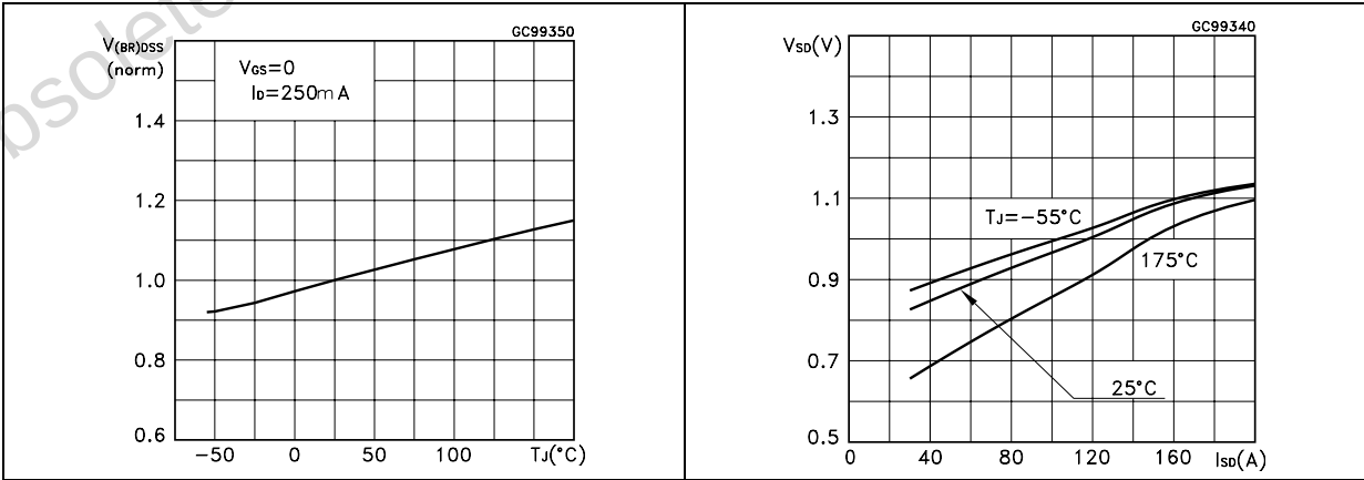
Figure 11. Normalized B_{V_{DS}} vs temperature Figure 12. Source-drain diode forward characteristics
