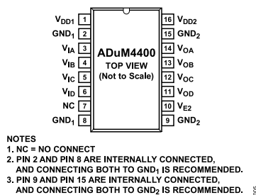
Figure 5. ADuM4400 Pin Configuration
