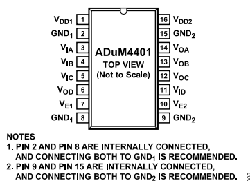
Figure 6. ADuM4401 Pin Configuration
