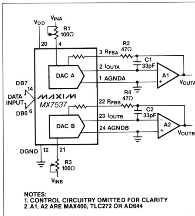
Figure 4A. MX7537 Unipolar Binary Operation
