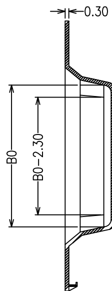
SECTION B-B
