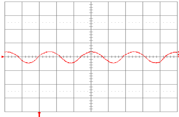
Fig. 2.0V.9: Input reflected ripple current, i_c (100 mA/div.), measured at input terminals at full rated load current and V_{in} = 48 \text{ V} . Refer to Fig. 2.0V.8 for test setup. Time scale: 1 \mu\text{s}/\text{div} .
