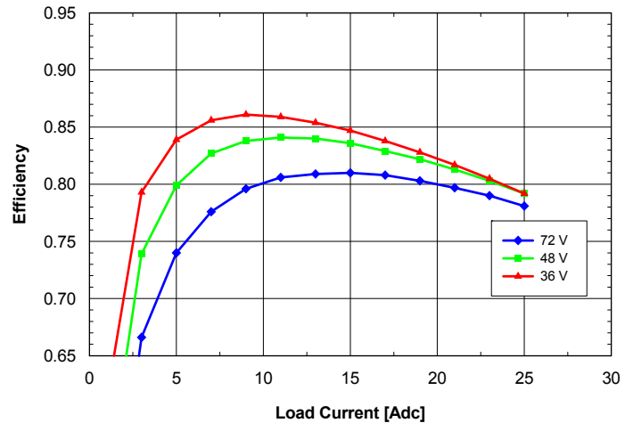
Fig. 1.2V.2: Efficiency vs. load current and input voltage for SQM48T/S25012 converter mounted vertically with air flowing from pin 3 to pin 1 at a rate of 300 LFM (1.5 m/s) and T_A = 25^{\circ}\text{C} .
