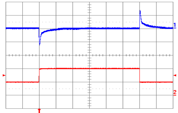
Fig. 2.0V.6: Output voltage response to load current step-change (5 A – 10 A – 5 A) at V_{in} = 48\text{ V} . Top trace: output voltage (100 mV/div.). Bottom trace: load current (5 A/div.). Current slew rate: 5 A/ \mu\text{s} . C_o = 450\text{ }\mu\text{F} tantalum + 1 \mu\text{F} ceramic. Time scale: 0.2 ms/div.
