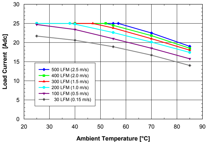
Fig. 1.8V.1: Available load current vs. ambient air temperature and airflow rates for SQM48T25018 converter with D height pins mounted vertically with air flowing from pin 3 to pin 1, MOSFET temperature \leq 120^{\circ}\text{C} , V_{in} = 48\text{ V} .
