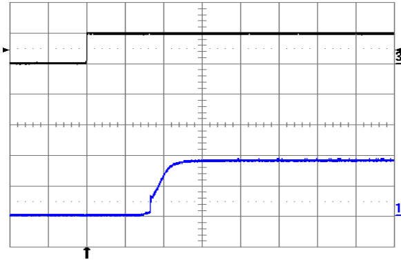
Fig. 1.8V.3: Turn-on transient at full rated load current (resistive) with no output capacitor at V_{in} = 48 V, triggered via ON/OFF pin. Top trace: ON/OFF signal (5 V/div.). Bottom trace: output voltage (1 V/div.). Time scale: 1 ms/div.
