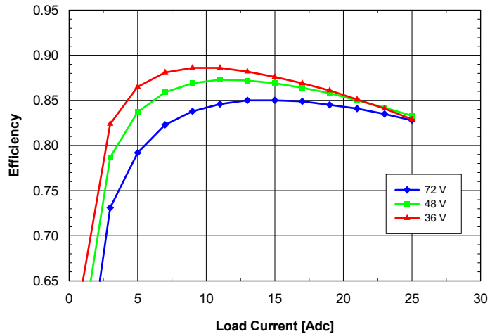
Fig. 1.8V.2: Efficiency vs. load current and input voltage for SQM48T/S25018 converter mounted vertically with air flowing from pin 3 to pin 1 at a rate of 300 LFM (1.5 m/s) and T_A = 25^{\circ}\text{C} .
