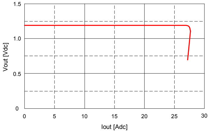
Fig. 1.2V.11: Output voltage vs. load current showing current limit point and converter shutdown point. Input voltage has almost no effect on current limit characteristic.
