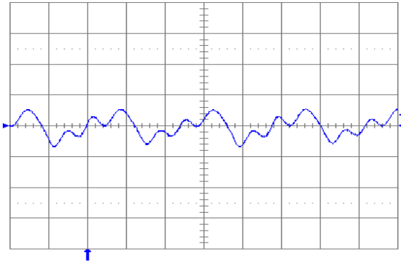
Fig. 1.8V.7: Output voltage ripple (20 mV/div.) at full rated load current into a resistive load with C_o = 10\ \mu\text{F} tantalum + 1\ \mu\text{F} ceramic and V_{in} = 48\ \text{V} . Time scale: 1\ \mu\text{s}/\text{div} .
