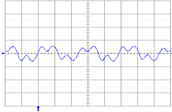
Fig. 2.5V.7: Output voltage ripple (20 mV/div.) at full rated load current into a resistive load with C_o = 10 \mu\text{F} tantalum + 1\mu\text{F} ceramic and V_{in} = 48 \text{ V} . Time scale: 1 \mu\text{s}/\text{div} .
