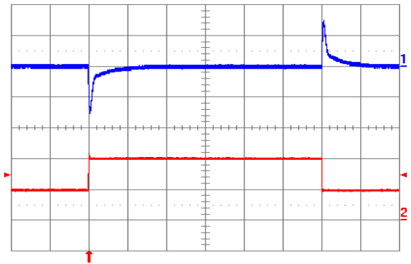
Fig. 1.5V.6: Output voltage response to load current step-change (5 A – 10 A – 5 A) at V_{in} = 48\text{ V} . Top trace: output voltage (100 mV/div.). Bottom trace: load current (5 A/div.). Current slew rate: 5 A/ \mu\text{s} . C_o = 450\text{ }\mu\text{F} tantalum + 1 \mu\text{F} ceramic. Time scale: 0.2 ms/div.
