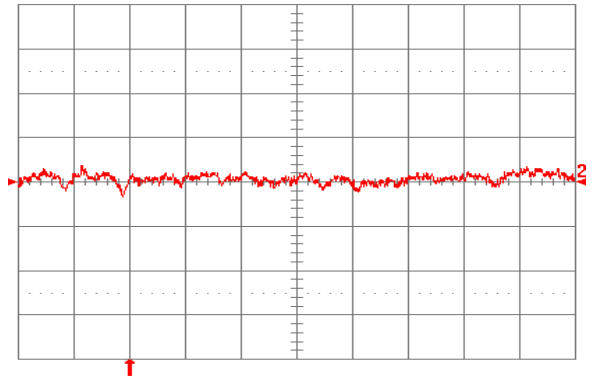
Fig. 1.5V.10: Input reflected ripple current, i_s (10 mA/div.), measured through 10 \mu\text{H} at the source at full rated load current and V_{in} = 48 \text{ V} . Refer to Fig 1.5V.8 for test setup. Time scale: 1 \mu\text{s}/\text{div} .
