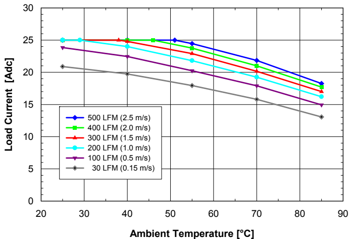
Fig. 2.0V.1: Available load current vs. ambient air temperature and airflow rates for SQM48T/S25020 converter with D height pins mounted vertically with air flowing from pin 3 to pin 1, MOSFET temperature \leq 120^\circ\text{C} , V_{in} = 48\text{ V} .
