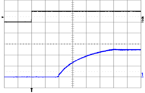
Fig. 2.5V.4: Turn-on transient at full rated load current (resistive) plus 20,000 \mu F at V_{in} = 48 V, triggered via ON/OFF pin. Top trace: ON/OFF signal (5 V/div.). Bottom trace: output voltage (1 V/div.). Time scale: 2 ms/div.
