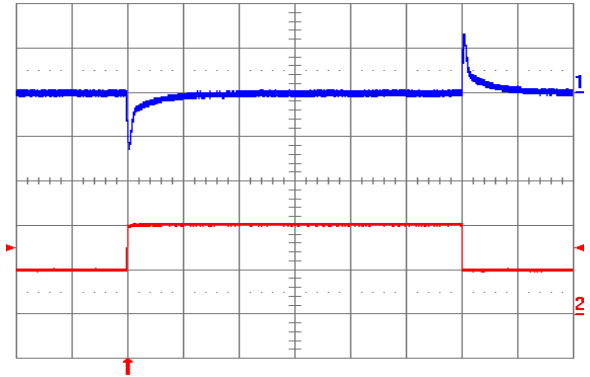
Fig. 2.5V.6: Output voltage response to load current step-change (5 A – 10 A – 5 A) at V_{in} = 48 V. Top trace: output voltage (100 mV/div.). Bottom trace: load current (5 A/div.). Current slew rate: 5 A/ \mu s. C_o = 450 \mu F tantalum + 1 \mu F ceramic. Time scale: 0.2 ms/div.
