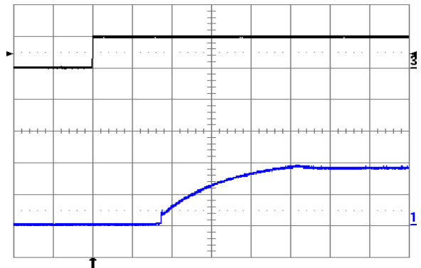
Fig. 1.8V.4: Turn-on transient at full rated load current (resistive) plus 20,000 \mu F at V_{in} = 48 V, triggered via ON/OFF pin. Top trace: ON/OFF signal (5 V/div.). Bottom trace: output voltage (1 V/div.). Time scale: 1 ms/div.
