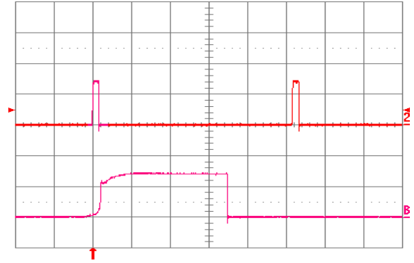
Fig. 1.2V.12: Load current (top trace, 20 A/div., 20 ms/div.) into a 10 mΩ short circuit during restart, at V_{in} = 48 V. Bottom trace (20 A/div., 1 ms/div.) is an expansion of the on-time portion of the top trace..
