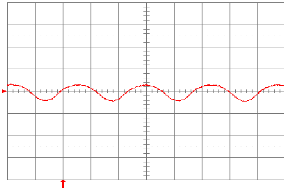
Fig. 1.5V.9: Input reflected ripple current, i_c (100 mA/div.), measured at input terminals at full rated load current and V_{in} = 48 \text{ V} . Refer to Fig. 1.5V.8 for test setup. Time scale: 1 \mu\text{s}/\text{div} .
