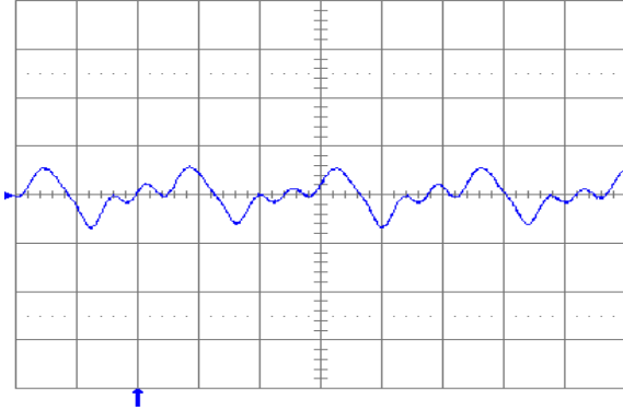
Fig. 1.5V.7: Output voltage ripple (20 mV/div.) at full rated load current into a resistive load with C_o = 10 \mu\text{F} tantalum + 1\mu\text{F} ceramic and V_{in} = 48 \text{ V} . Time scale: 1 \mu\text{s}/\text{div} .
