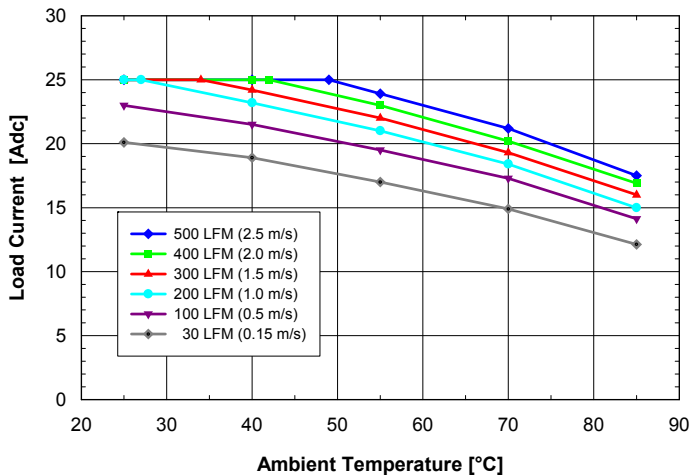
Fig. 2.5V.1: Available load current vs. ambient air temperature and airflow rates for SQM48T25025 converter with D height pins mounted vertically with air flowing from pin 3 to pin 1, MOSFET temperature \leq 120^\circ\text{C} , V_{in} = 48\text{ V} .
