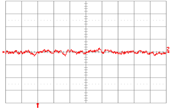
Fig. 2.5V.10: Input reflected ripple current, i_s (10 mA/div.), measured through 10 \mu\text{H} at the source at full rated load current and V_{in} = 48 \text{ V} . Refer to Fig. 2.5V.8 for test setup. Time scale: 1 \mu\text{s}/\text{div} .
