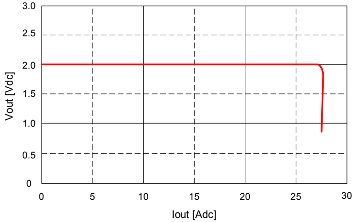
Fig. 2.0V.11: Output voltage vs. load current showing current limit point and converter shutdown point. Input voltage has almost no effect on current limit characteristic.
