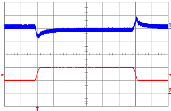
Fig. 1.8V.5: Output voltage response to load current step-change (5 A – 10 A – 5 A) at V_{in} = 48 V. Top trace: output voltage (100 mV/div.). Bottom trace: load current (5 A/div.). Current slew rate: 0.1 A/ \mu s. C_o = 1 \mu F ceramic. Time scale: 0.2 ms/div.
