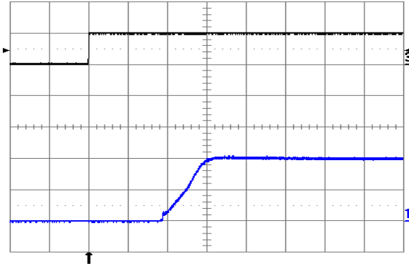
Fig. 2.0V.3: Turn-on transient at full rated load current (resistive) with no output capacitor at V_{in} = 48\text{ V} , triggered via ON/OFF pin. Top trace: ON/OFF signal (5 V/div.). Bottom trace: output voltage (1 V/div.). Time scale: 1 ms/div.
