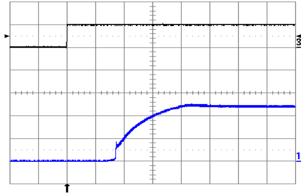
Fig. 1.2V.4: Turn-on transient at full rated load current (resistive) plus 20,000 \mu\text{F} at V_{in} = 48\text{ V} , triggered via ON/OFF pin. Top trace: ON/OFF signal (5 V/div.). Bottom trace: output voltage (0.5 V/div.). Time scale: 1 ms/div.
