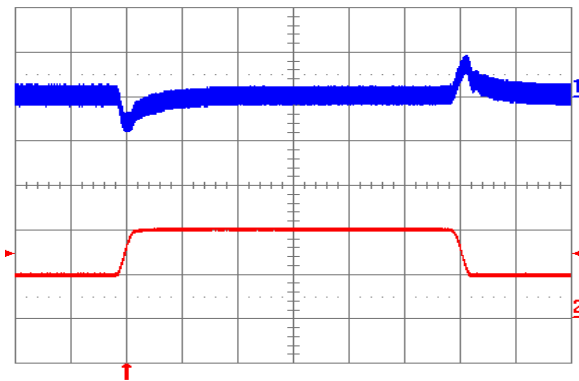
Fig. 1.2V.5: Output voltage response to load current step-change (5 A – 10 A – 5 A) at V_{in} = 48\text{ V} . Top trace: output voltage (100 mV/div.). Bottom trace: load current (5 A/div.). Current slew rate: 0.1 A/ \mu\text{s} . C_o = 1\text{ }\mu\text{F} ceramic. Time scale: 0.2 ms/div.
