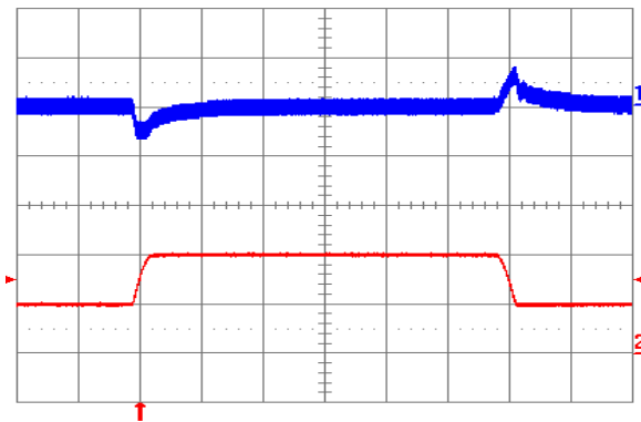
Fig. 2.0V.5: Output voltage response to load current step-change (5 A – 10 A – 5 A) at V_{in} = 48\text{ V} . Top trace: output voltage (100 mV/div.). Bottom trace: load current (5 A/div.). Current slew rate: 0.1 A/ \mu\text{s} . C_o = 1\text{ }\mu\text{F} ceramic. Time scale: 0.2 ms/div.
