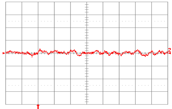
Fig. 1.8V.10: Input reflected ripple current, i_s (10 mA/div.), measured through 10\ \mu\text{H} at the source at full rated load current and V_{in} = 48\ \text{V} . Refer to Fig. 1.8V.8 for test setup. Time scale: 1\ \mu\text{s}/\text{div} .
