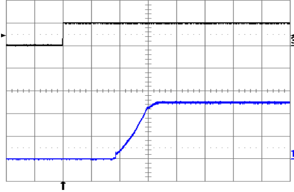
Fig. 2.5V.3: Turn-on transient at full rated load current (resistive) with no output capacitor at V_{in} = 48 V, triggered via ON/OFF pin. Top trace: ON/OFF signal (5 V/div.). Bottom trace: output voltage (1 V/div.). Time scale: 1 ms/div.
