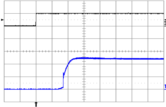
Fig. 1.2V.3: Turn-on transient at full rated load current (resistive) with no output capacitor at V_{in} = 48\text{ V} , triggered via ON/OFF pin. Top trace: ON/OFF signal (5 V/div.). Bottom trace: output voltage (0.5 V/div.). Time scale: 1 ms/div.
