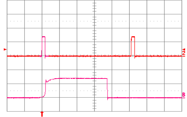
Fig. 1.5V.12: Load current (top trace, 20 A/div., 20 ms/div.) into a 10 mΩ short circuit during restart, at V_{in} = 48 V. Bottom trace (20 A/div., 1 ms/div.) is an expansion of the on-time portion of the top trace.
