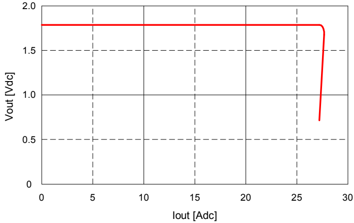
Fig. 1.8V.11: Output voltage vs. load current showing current limit point and converter shutdown point. Input voltage has almost no effect on current limit characteristic.
