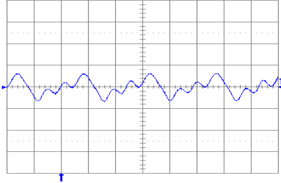
Fig. 2.0V.7: Output voltage ripple (20 mV/div.) at full rated load current into a resistive load with C_o = 10 \mu\text{F} tantalum + 1\mu\text{F} ceramic and V_{in} = 48 \text{ V} . Time scale: 1 \mu\text{s}/\text{div} .
