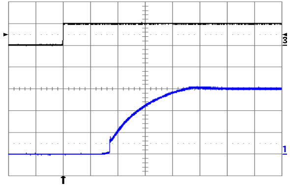
Fig. 1.5V.4: Turn-on transient at full rated load current (resistive) plus 20,000 \mu\text{F} at V_{in} = 48\text{ V} , triggered via ON/OFF pin. Top trace: ON/OFF signal (5 V/div.). Bottom trace: output voltage (0.5 V/div.). Time scale: 1 ms/div.
