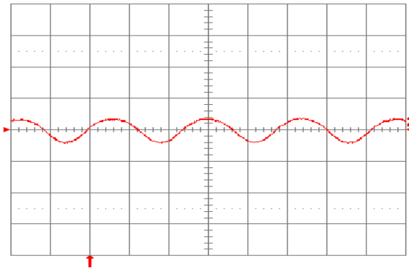
Fig. 1.8V.9: Input reflected ripple current, i_c (100 mA/div.), measured at input terminals at full rated load current and V_{in} = 48\ \text{V} . Refer to Fig. 1.8V.8 for test setup. Time scale: 1\ \mu\text{s}/\text{div} .
