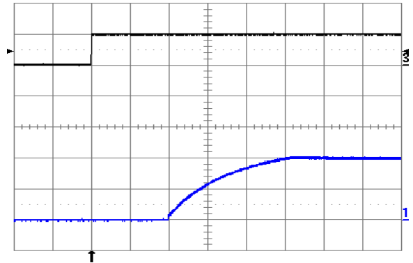
Fig. 2.0V.4: Turn-on transient at full rated load current (resistive) plus 20,000 \mu\text{F} at V_{in} = 48\text{ V} , triggered via ON/OFF pin. Top trace: ON/OFF signal (5 V/div.). Bottom trace: output voltage (1 V/div.). Time scale: 1 ms/div.
