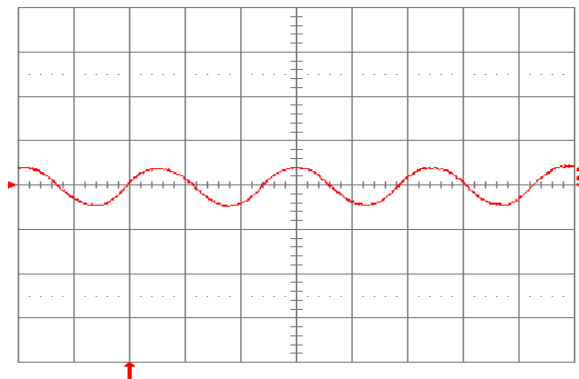
Fig. 2.5V.9: Input reflected ripple current, i_c (100 mA/div.), measured at input terminals at full rated load current and V_{in} = 48 \text{ V} . Refer to Fig. 2.5V.8 for test setup. Time scale: 1 \mu\text{s}/\text{div} .
