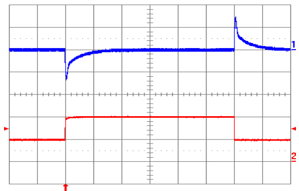
Fig. 1.8V.6: Output voltage response to load current step-change (5 A – 10 A – 5 A) at V_{in} = 48 V. Top trace: output voltage (100 mV/div.). Bottom trace: load current (5 A/div.). Current slew rate: 5 A/ \mu s. C_o = 450 \mu F tantalum + 1 \mu F ceramic. Time scale: 0.2 ms/div.
