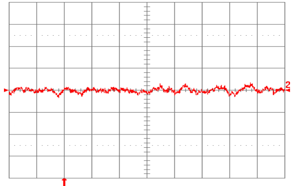
Fig. 2.0V.10: Input reflected ripple current, i_s (10 mA/div.), measured through 10 \mu\text{H} at the source at full rated load current and V_{in} = 48 \text{ V} . Refer to Fig. 2.0V.8 for test setup. Time scale: 1 \mu\text{s}/\text{div} .
