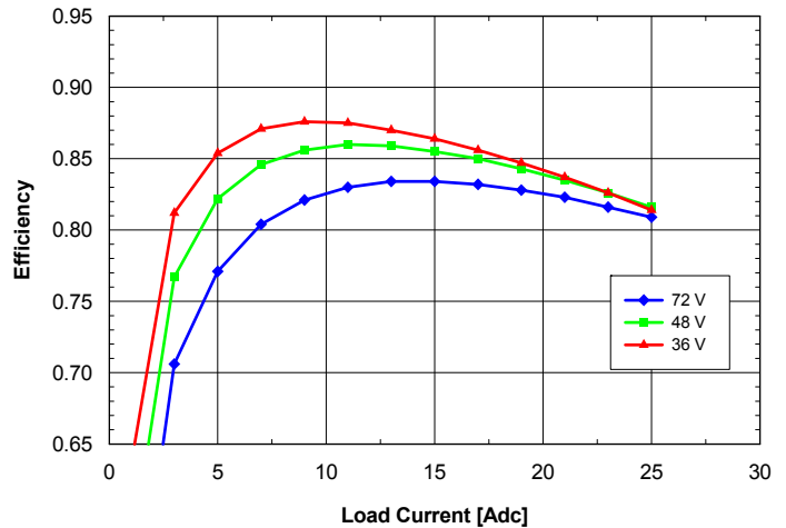
Fig. 1.5V.2: Efficiency vs. load current and input voltage for SQM48T/S25015 converter mounted vertically with air flowing from pin 3 to pin 1 at a rate of 300 LFM (1.5 m/s) and T_a = 25^{\circ}\text{C} .
