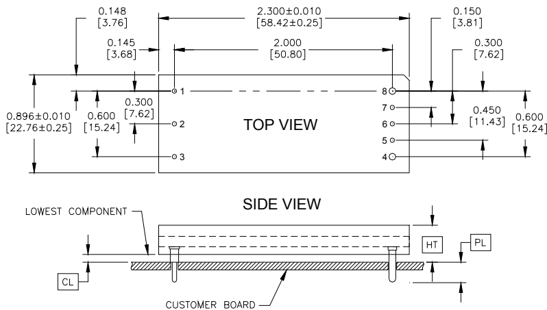
SQM48T Pinout (Through-hole)
