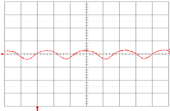
Fig. 1.2V.9: Input reflected ripple current, i_c (100 mA/div.), measured at input terminals at full rated load current and V_{in} = 48 \text{ V} . Refer to Fig. 1.2V.8 for test setup. Time scale: 1 \mu\text{s}/\text{div} .
