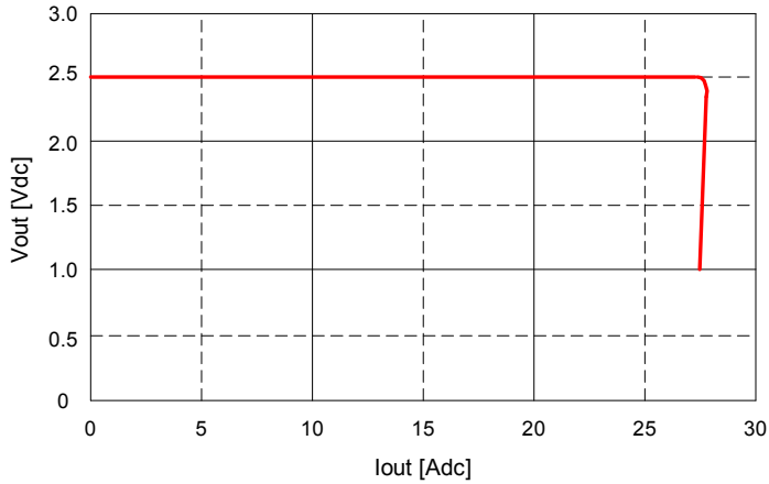
Fig. 2.5V.11: Output voltage vs. load current showing current limit point and converter shutdown point. Input voltage has almost no effect on current limit characteristic.
