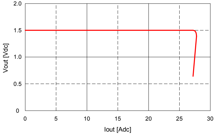
Fig. 1.5V.11: Output voltage vs. load current showing current limit point and converter shutdown point. Input voltage has almost no effect on current limit characteristic.
