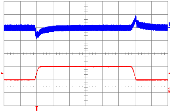
Fig. 2.5V.5: Output voltage response to load current step-change (5 A – 10 A – 5 A) at V_{in} = 48 V. Top trace: output voltage (100 mV/div.). Bottom trace: load current (5 A/div.). Current slew rate: 0.1 A/ \mu s. C_o = 1 \mu F ceramic. Time scale: 0.2 ms/div.
