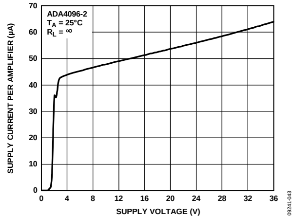
Figure 42. Supply Current vs. Supply Voltage
