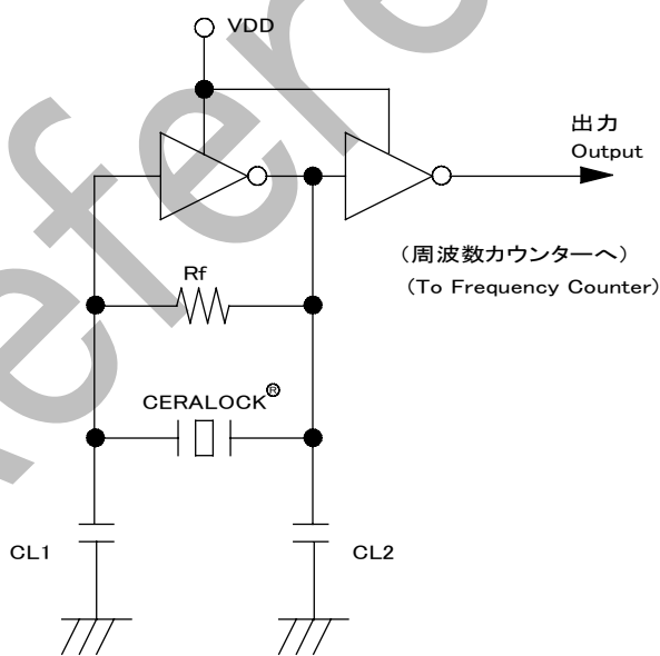
Figure 2. Test Circuit
