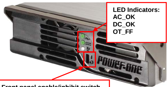
FXP series front bezel showing LED indicators and recessed enable switch
