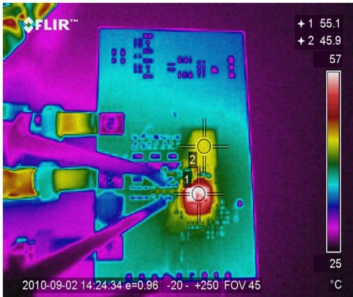
Figure 31: Thermal Image of the board at 25A load Test point 1 is iP1827 Test point 2 is inductor
