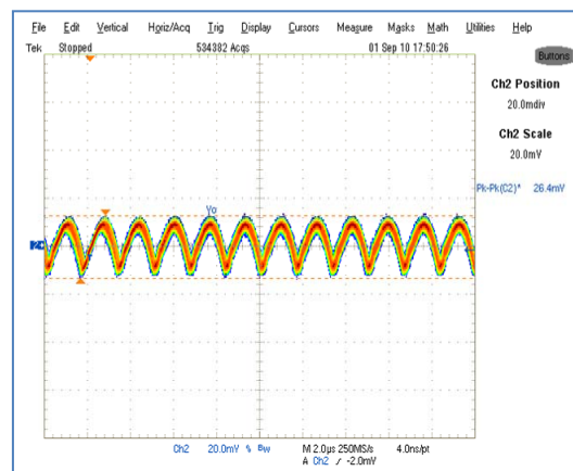
Figure 23: Output Voltage Ripple, 25A load Ch2: V_{out}
