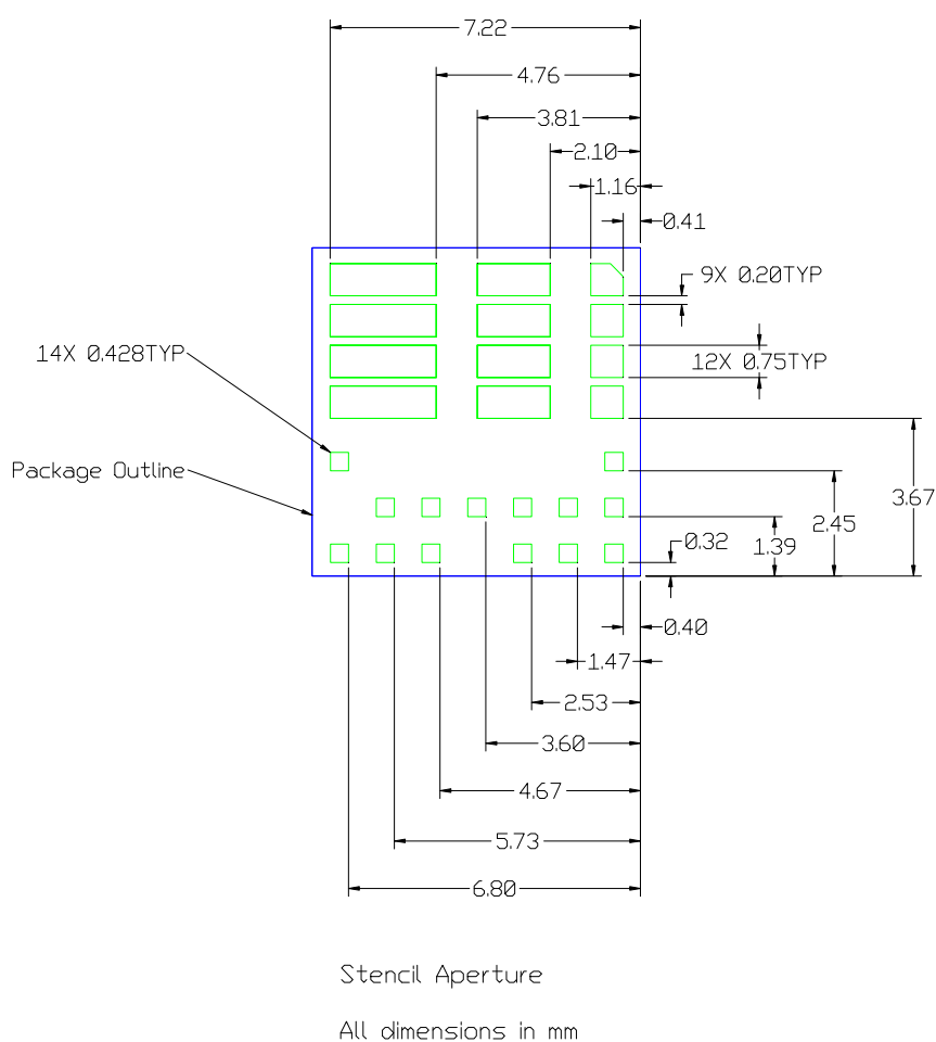
Figure 38: Stencil design
