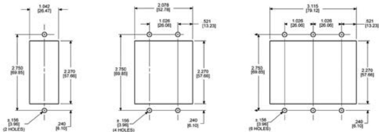
Mounting Details
