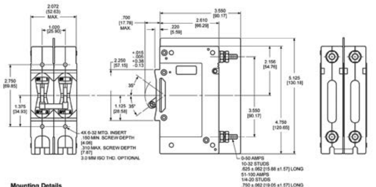
Mounting Details
