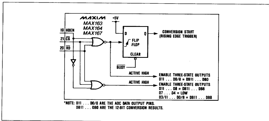
Figure 8. Logic Equivalent for \overline{\text{RD}} , \overline{\text{CS}} and HBEN Inputs
