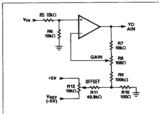
Figure 17. Offset ( \pm 20\text{mV} ) and Gain ( \pm 0.5\% ) Trim Circuit
