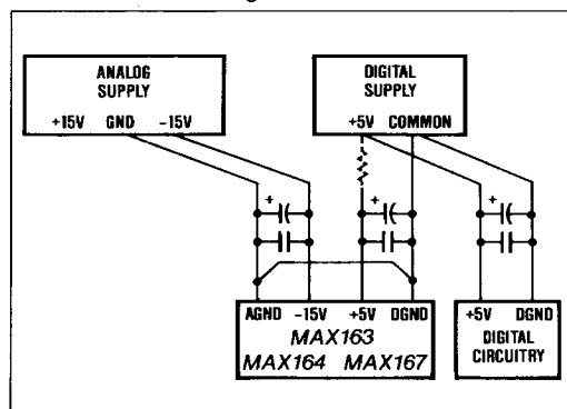
Figure 13. Power Supply Grounding Practice
