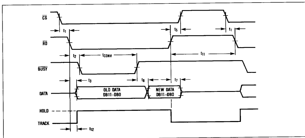
Figure 9. Slow Memory Mode, Parallel Read Timing Diagram
