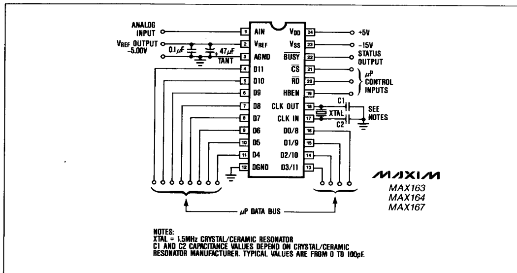
Figure 3. MAX163/164/167 Operational Diagram
