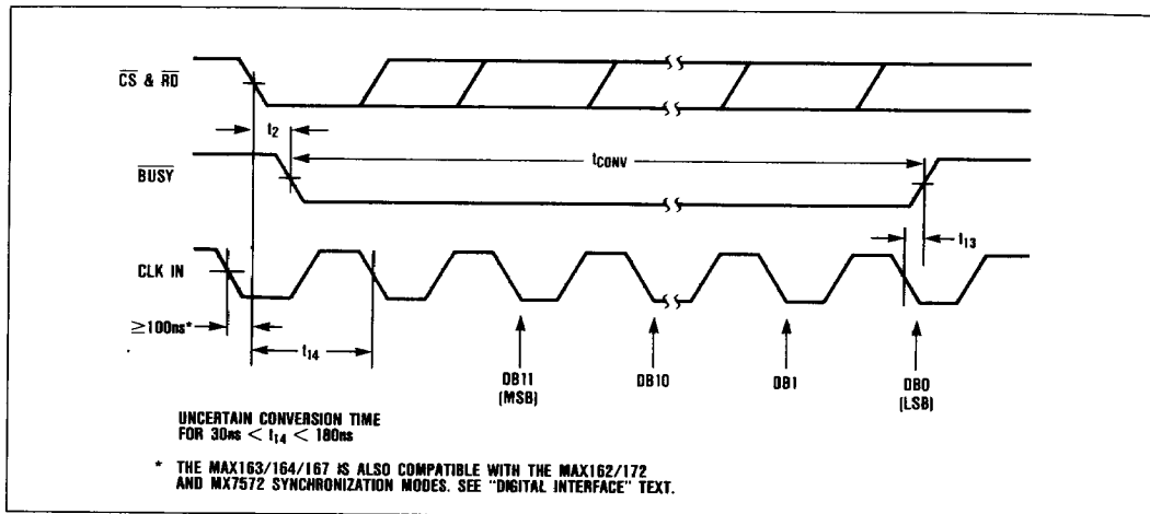
Figure 7. \overline{\text{RD}} and CLK IN for Synchronous Operation
