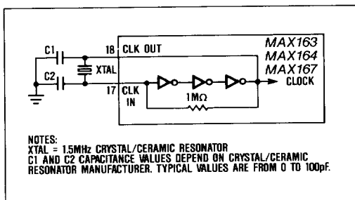
Figure 6. Internal Clock Circuit
