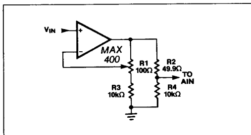
Figure 16. Trim Circuit for Gain Only ( \pm 0.5\% )
