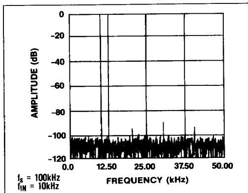
Figure 18. FFT Plot for the MAX167
