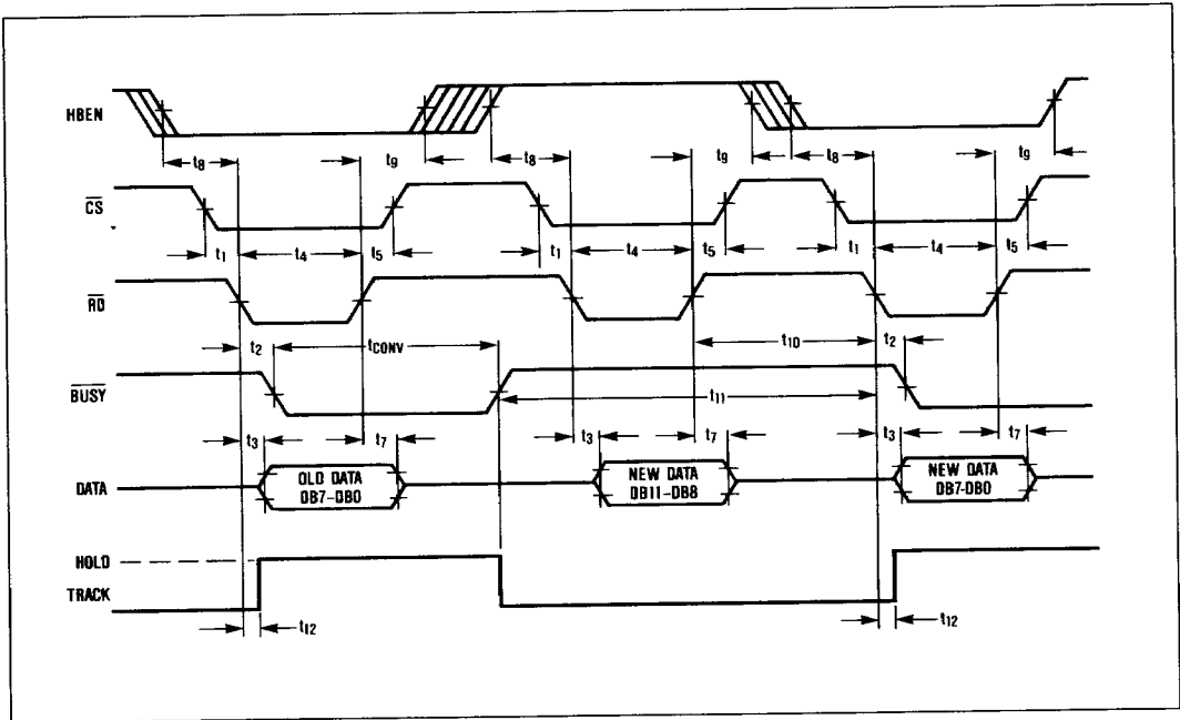
Figure 12. ROM Mode, Two Byte Read Timing Diagram
