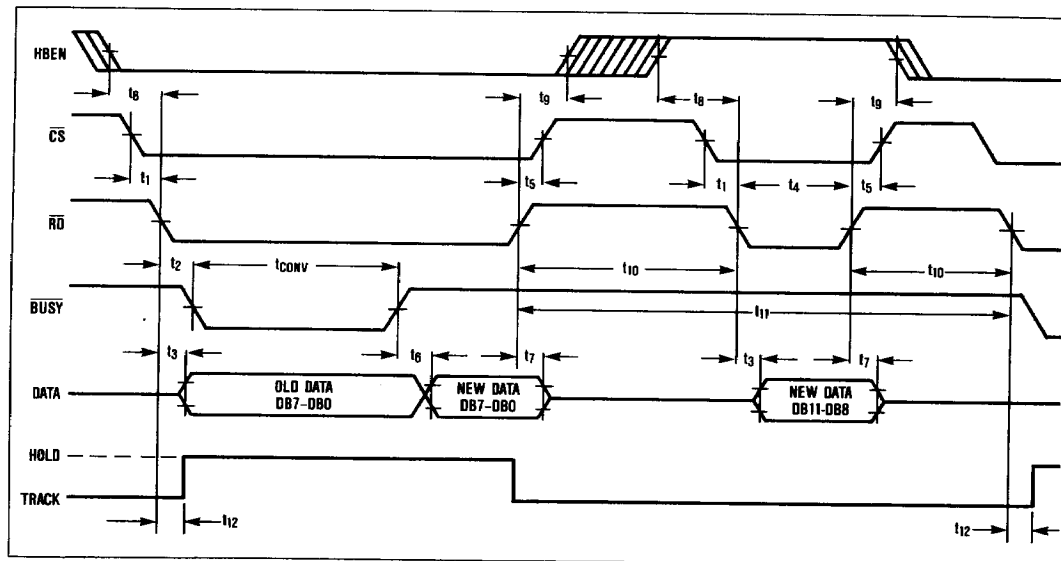
Figure 10. Slow Memory Mode, Two Byte Read Timing Diagram
