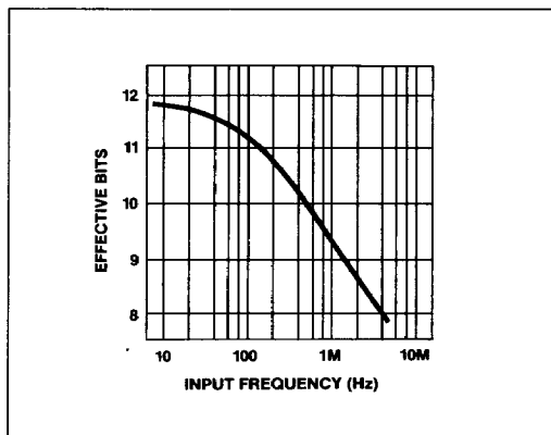
Figure 19. MAX167 Effective Bits vs. Input Frequency
