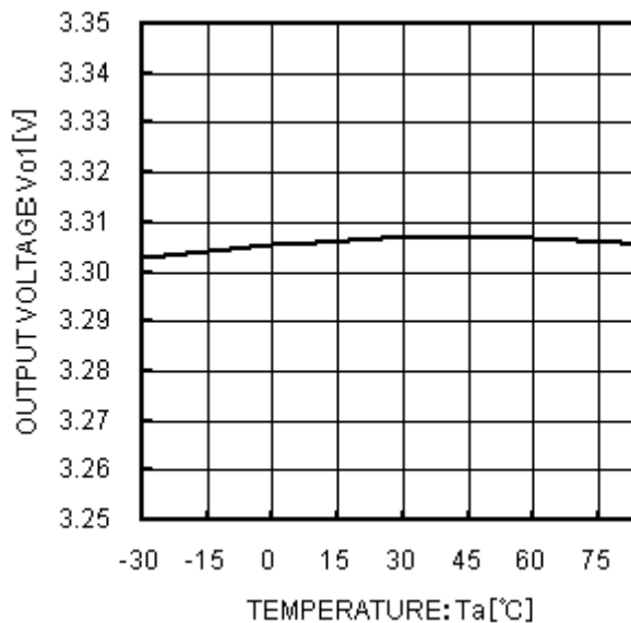
Fig.12 Output Voltage vs Temperature (3.3 V output)
