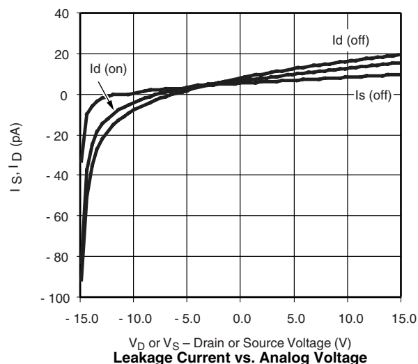
Leakage Current vs. Analog Voltage
