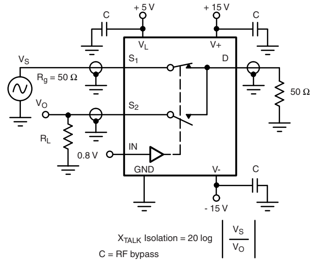
Figure 7. Crosstalk
