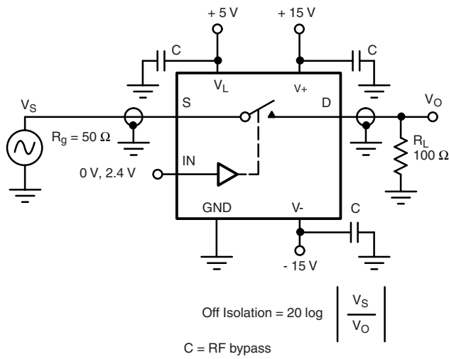
Figure 5. Off Isolation
