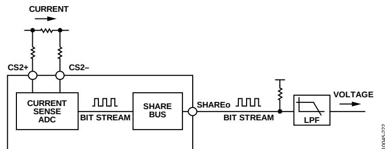
Figure 32. Analog Current Share Configuration
