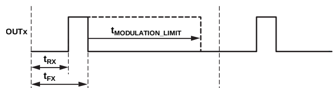
Figure 21. Modulation Limit Settings
