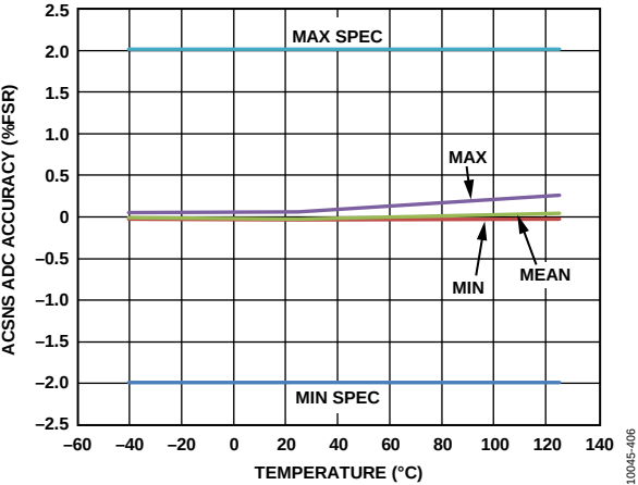
Figure 11. ACSNS ADC Accuracy vs. Temperature (from 10% to 90% of FSR)
