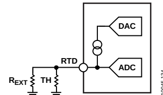
Figure 36. Temperature Measurement Using Thermistor
