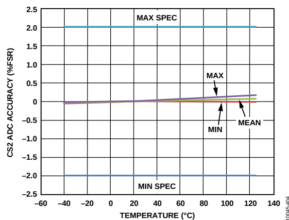
Figure 9. CS2 ADC Accuracy vs. Temperature (from 10% to 90% of FSR)
