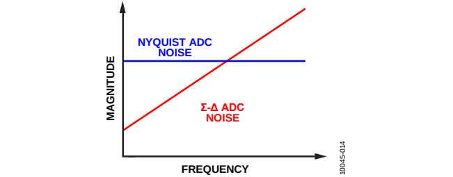
Figure 17. Noise Performance for Nyquist Rate and Σ-Δ ADCs
