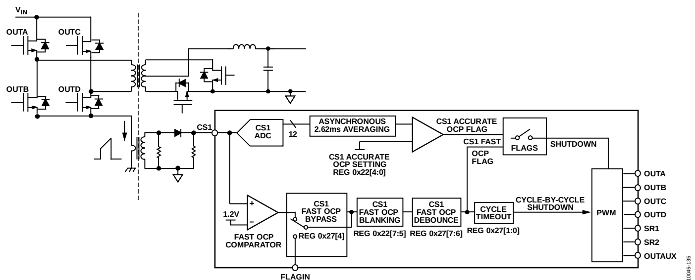
Figure 38. CS1 OCP Detailed Internal Schematic
