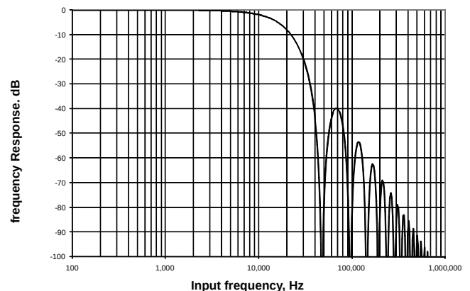
Figure 8-5. Delta-sigma ADC Frequency Response, Normalized to Output, Sample Rate = 48 kHz
