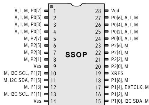
CY7C60323-PVXC Device
