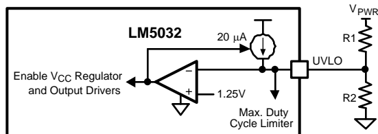
Figure 25. UVLO Circuit
