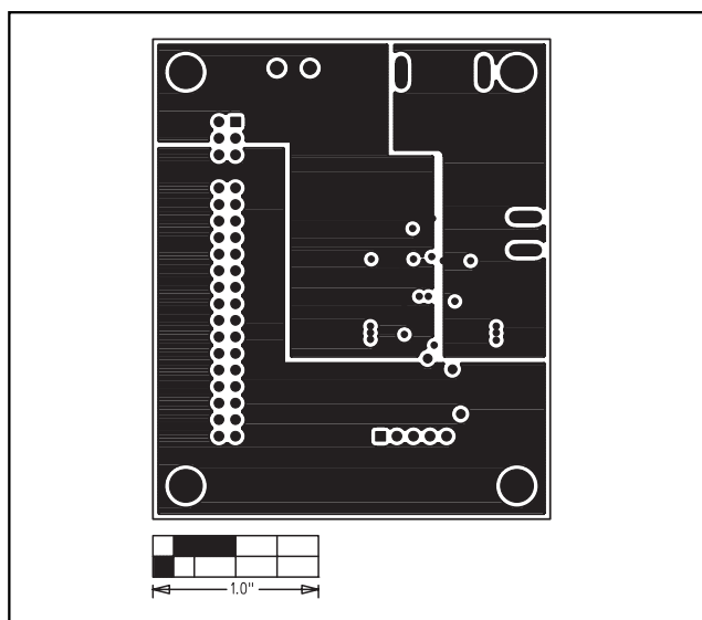
Figure 6. MAX1162 EV Kit PCB Layout—Inner Layer 3 (VDD)
