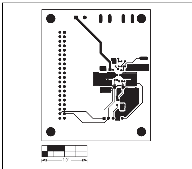
Figure 4. MAX1162 EV Kit PCB Layout—Component Side
