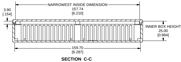
SECTION C-C
