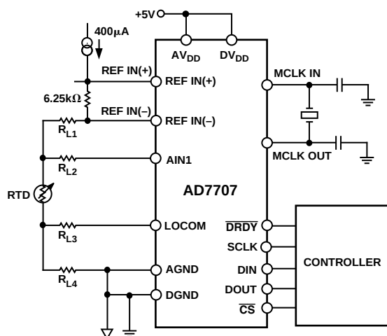
Figure 29. RTD Measurement Using the AD7707
