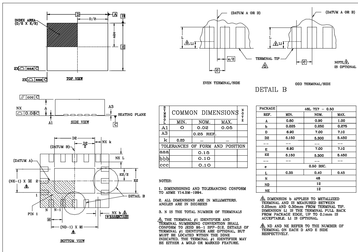
Figure 21. Package Drawing
