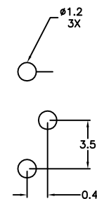
RECOMMENDED MOUNTING PATTERN
