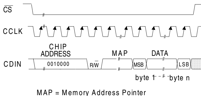
Figure 23. Control Port Timing, SPI mode
