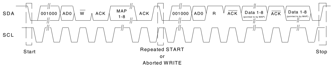
Figure 22. I²C Read
