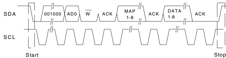
Figure 21. I²C Write
