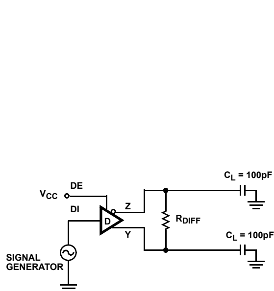
FIGURE 2A. TEST CIRCUIT
