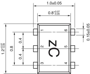
PACKAGE OUTLINE M16
