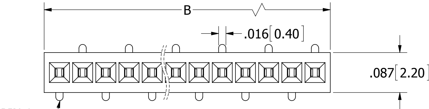
LPPB_1NFS-RC (OPPOSITE BEND, APPLICABLE ON EVEN PIN COUNTS)
