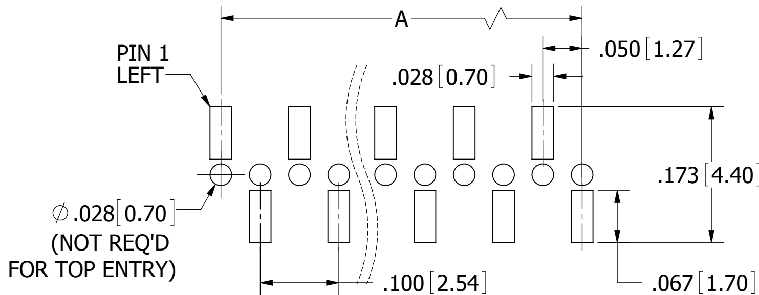
RECOMMENDED PCB LAYOUT LPPB_1NFS-RC
