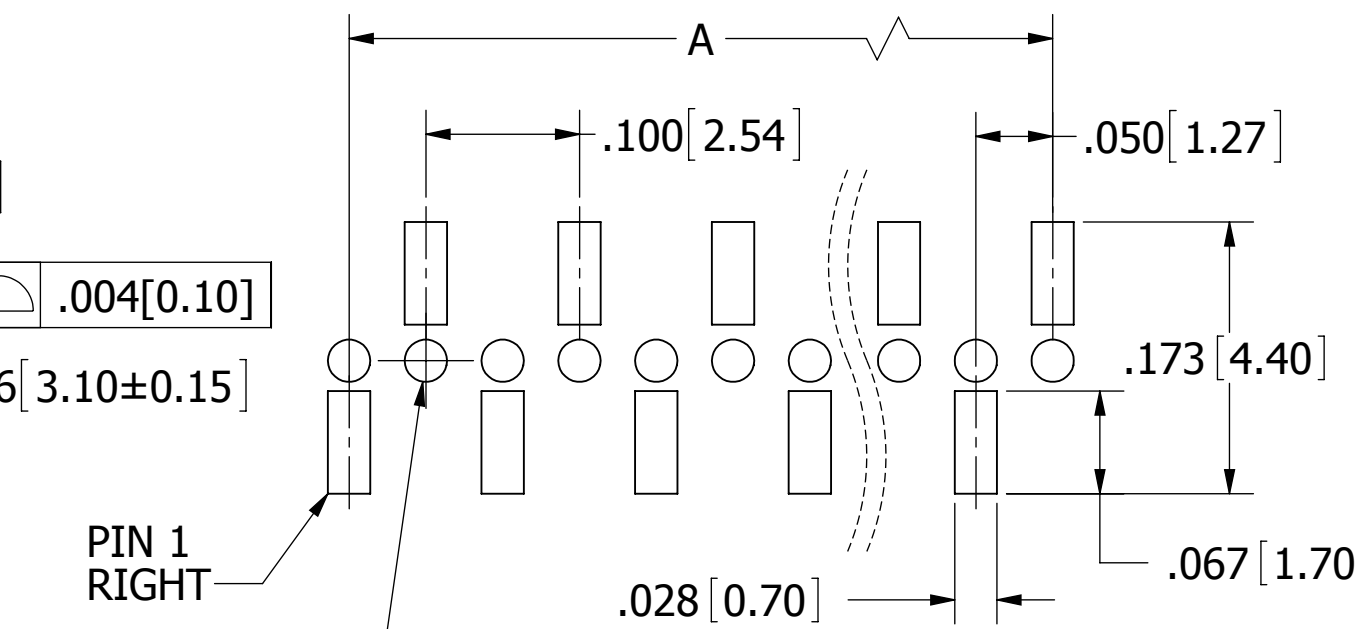
RECOMMENDED PCB LAYOUT LPPB_1NFS-RC
