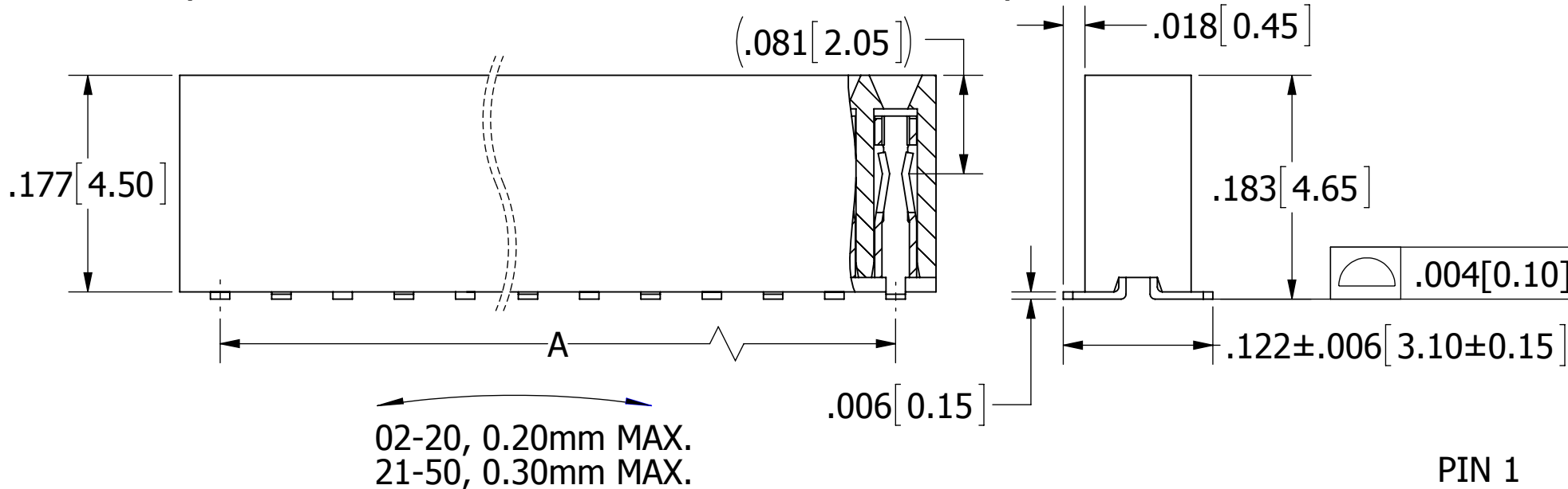
LPPB_1NFS-RC (OPPOSITE BEND, APPLICABLE ON EVEN PIN COUNTS)
