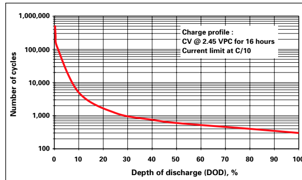
Figure 7-1: Cycle Life and DOD for CYCLON® Battery Cells
