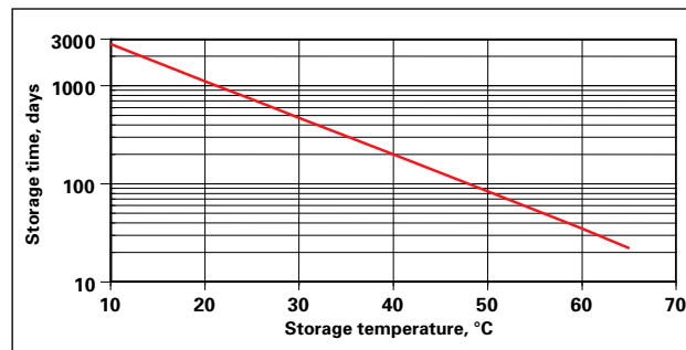
Figure 5-2: CYCLON® Battery Storage Time Vs. Temperature
