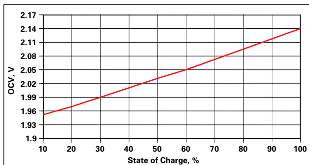
Figure 5-1: CYCLON® Battery Open Circuit Voltage Vs. State of Charge
