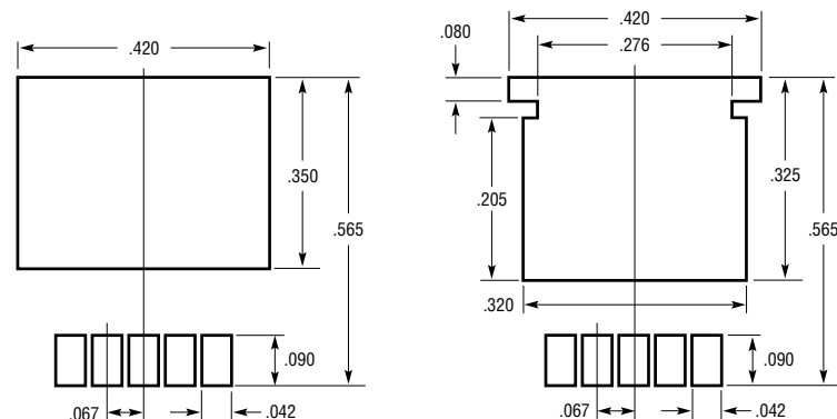
RECOMMENDED SOLDER PAD LAYOUT
