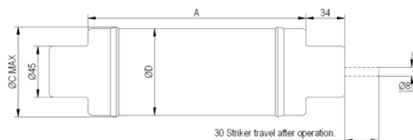
EJ Outline
