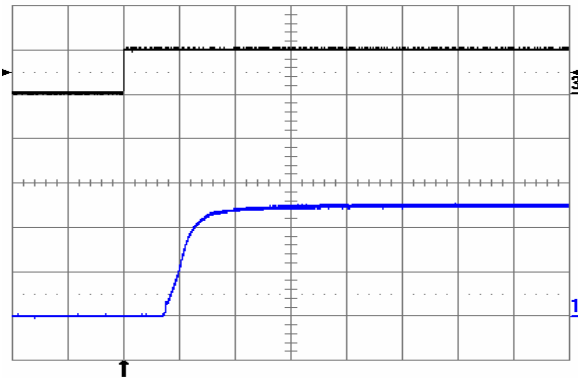
Fig. 5.0V.9: Turn-on transient at full rated load current (resistive) with no output capacitor at V_{in} = 48\text{ V} , triggered via ON/OFF pin. Top trace: ON/OFF signal (5 V/div.). Bottom trace: output voltage (2 V/div.). Time scale: 2 ms/div.
