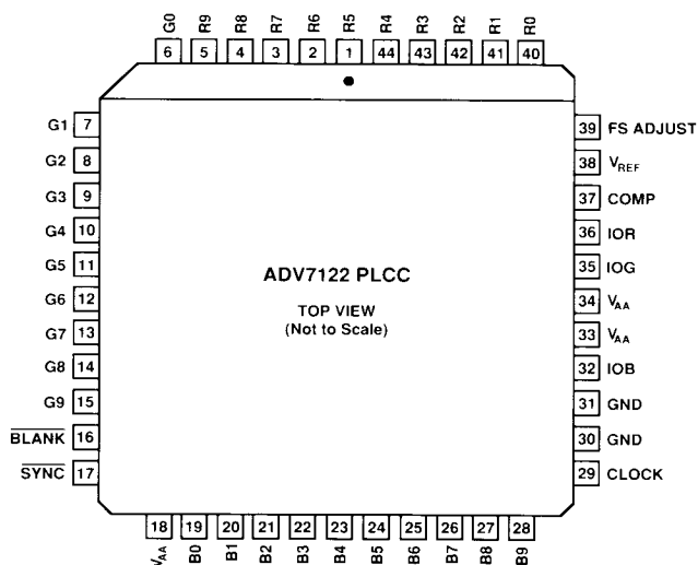
PLCC (P-44A) Package
