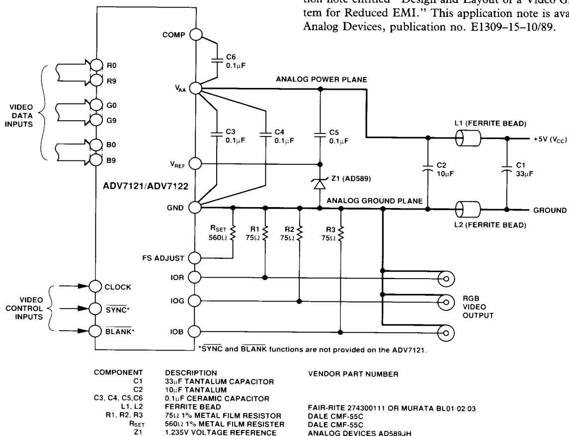
Figure 8. ADV7121/ADV7122 Typical Connection Diagram and Component List
