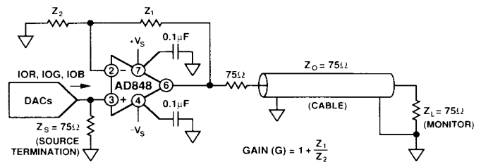
Figure 7. AD848 As an Output Buffer
