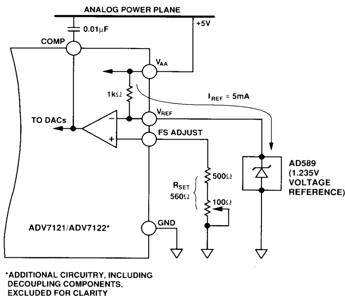
Figure 4. Reference Circuit
