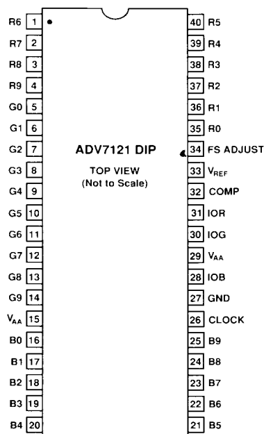
DIP (N-40A) Package
