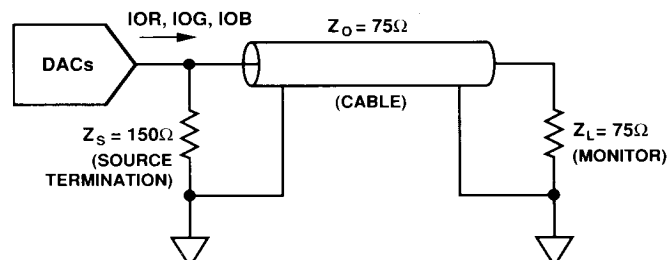
Figure 5a. Analog Output Termination for RS-343A
