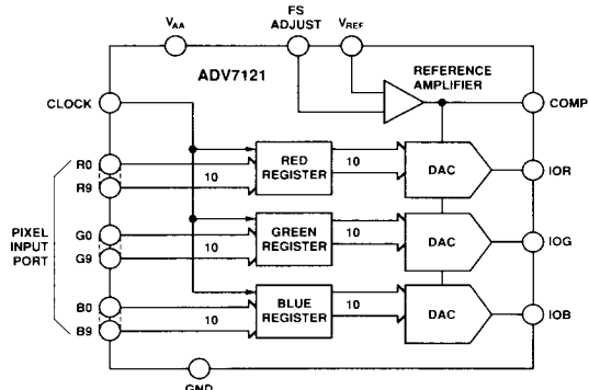
ADV7121 Functional Block Diagram
