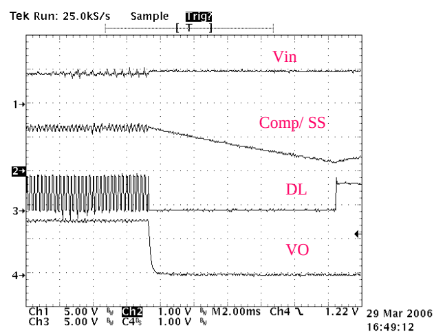
Over Current Protection (21A DC tripped)
