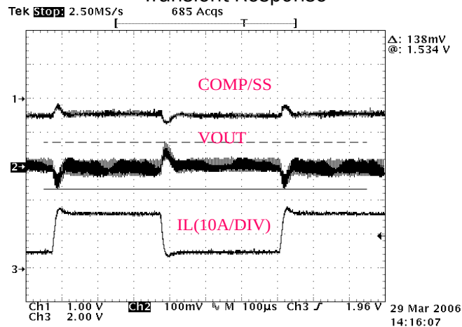
5 -18 A step load
