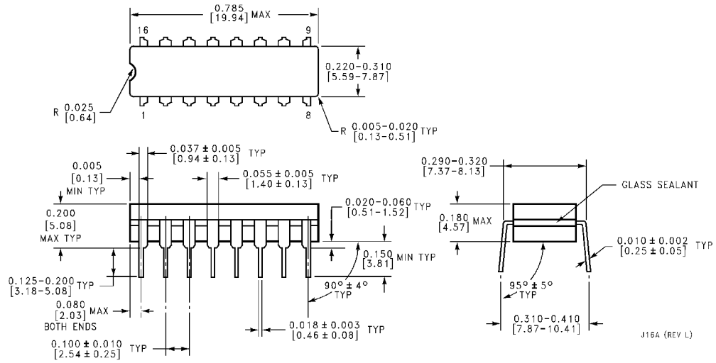
16-Lead Ceramic Dual-In-Line Package (J) Order Number DM54LS75J Package Number J16A
