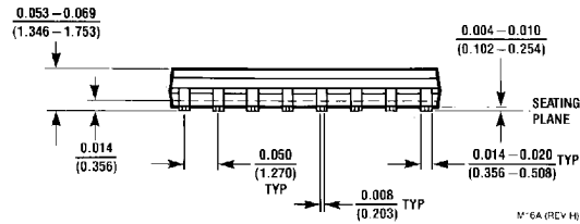
16-Lead Small Outline Molded Package (M) Order Number DM74LS75M Package Number M16A
