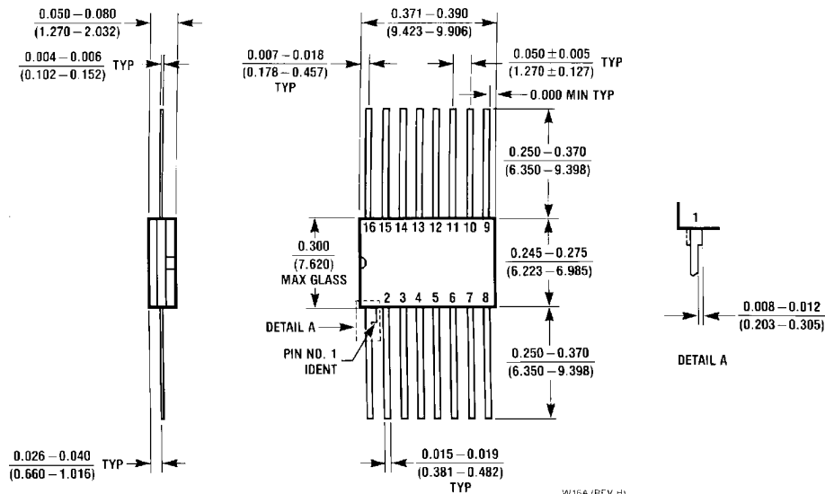
16-Lead Ceramic Flat Package (W) Order Number DM54LS75W Package Number W16A
