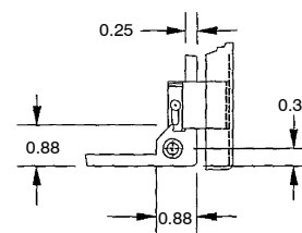
Hinge Detail
