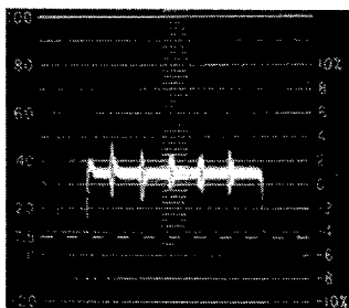
Differential Gain (Note)
