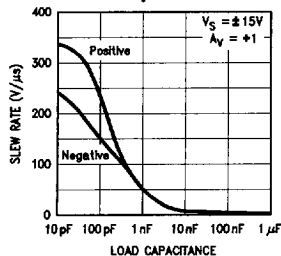
Slew Rate vs Load Capacitance
