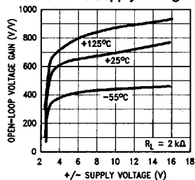
Gain vs Supply Voltage
