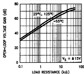
Voltage Gain vs Load Resistance
