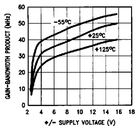
Gain-Bandwidth Product
