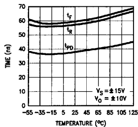
Propagation Delay Rise and Fall Times
