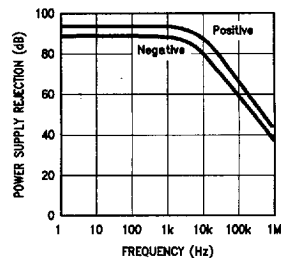
Power Supply Rejection Ratio
