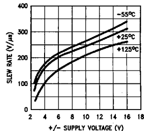
Slew Rate
